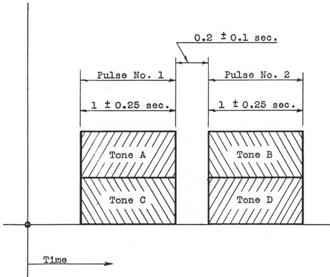
Figure: 2-2 SELCAL Code AB-CD Example
